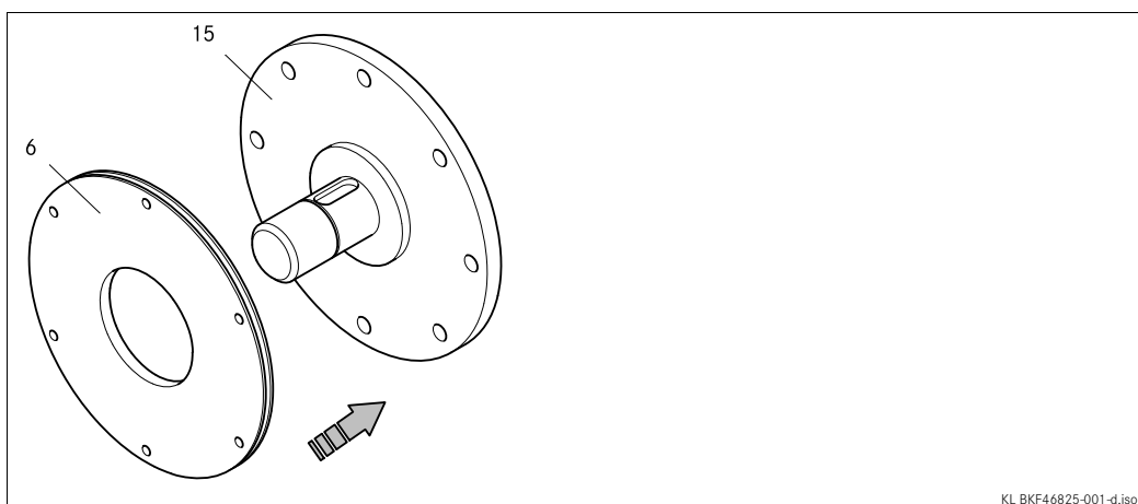
Abb. 6 Flanschmontage BFK468
