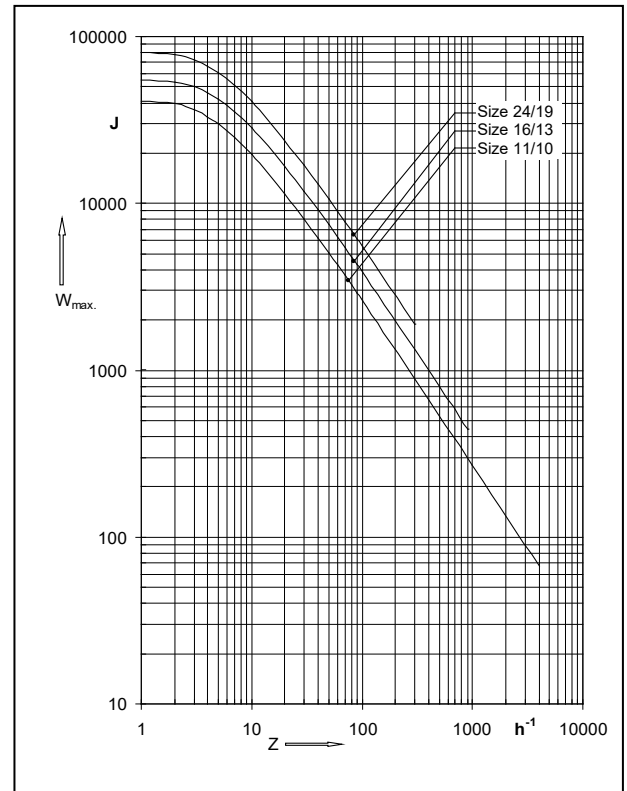
Fig. 33/1: Max. switching work W_{\max} per switching operation as a function of the number of switching operations per hour Z (values based on n=1500 rpm)
