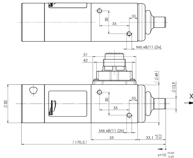
Dimension drawing
